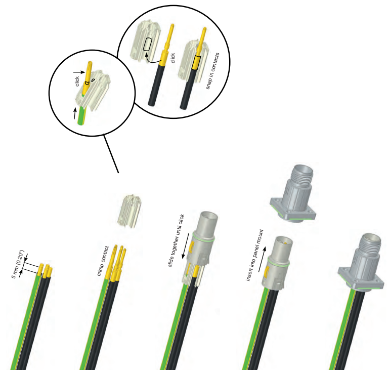
Panel Connector, K- / L-Coding (Crimp)
