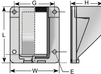
Flange Type 2: PG 29 - PG 48
