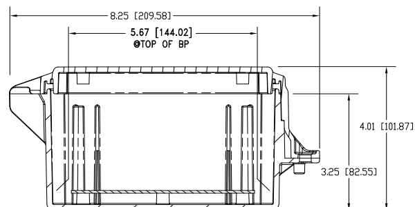
SECTION B-B
