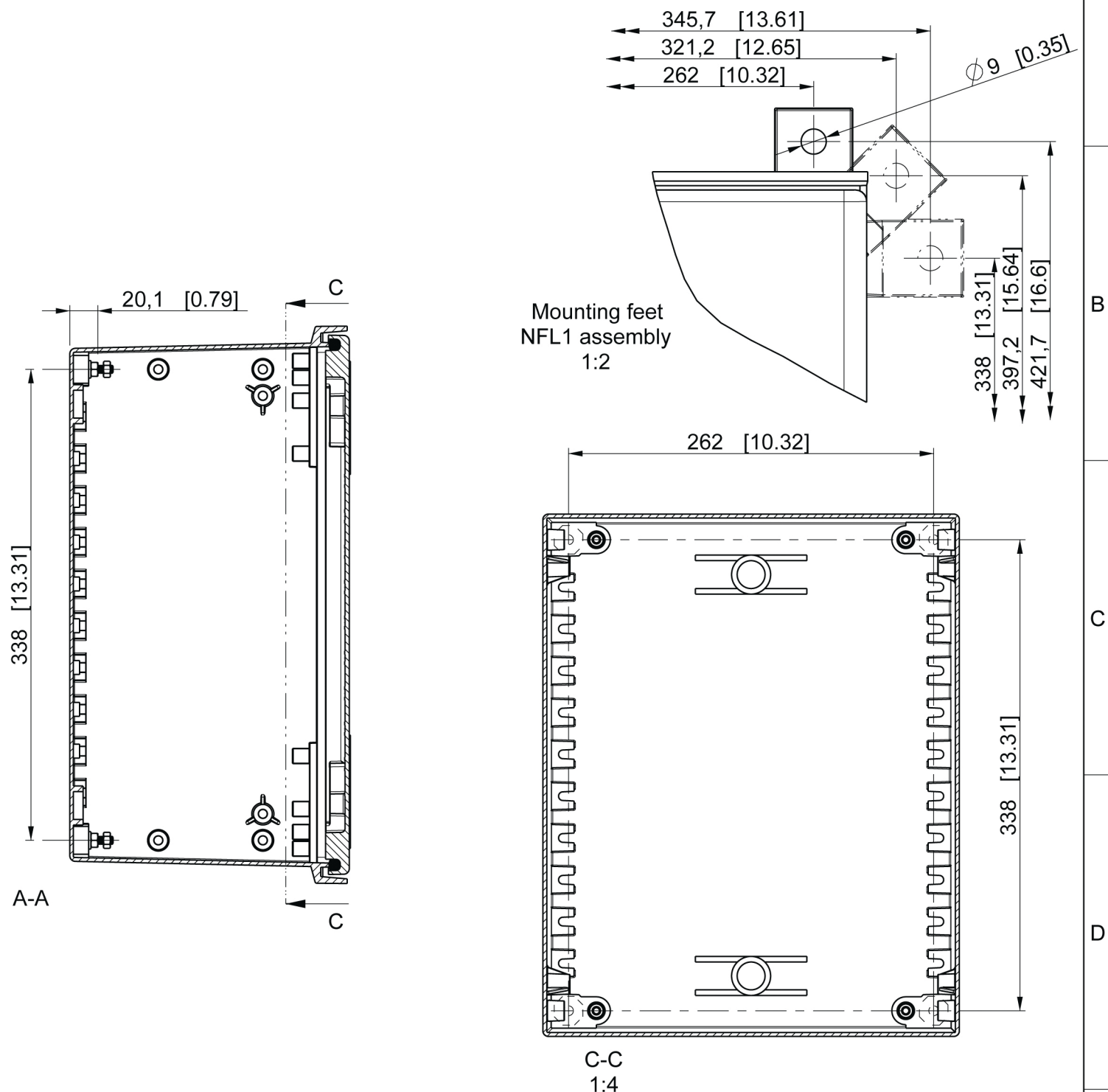
Dimensions in mm [inches]
